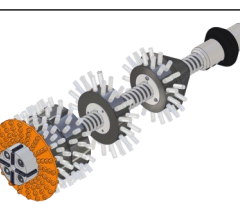
Twister Concrete Remover
