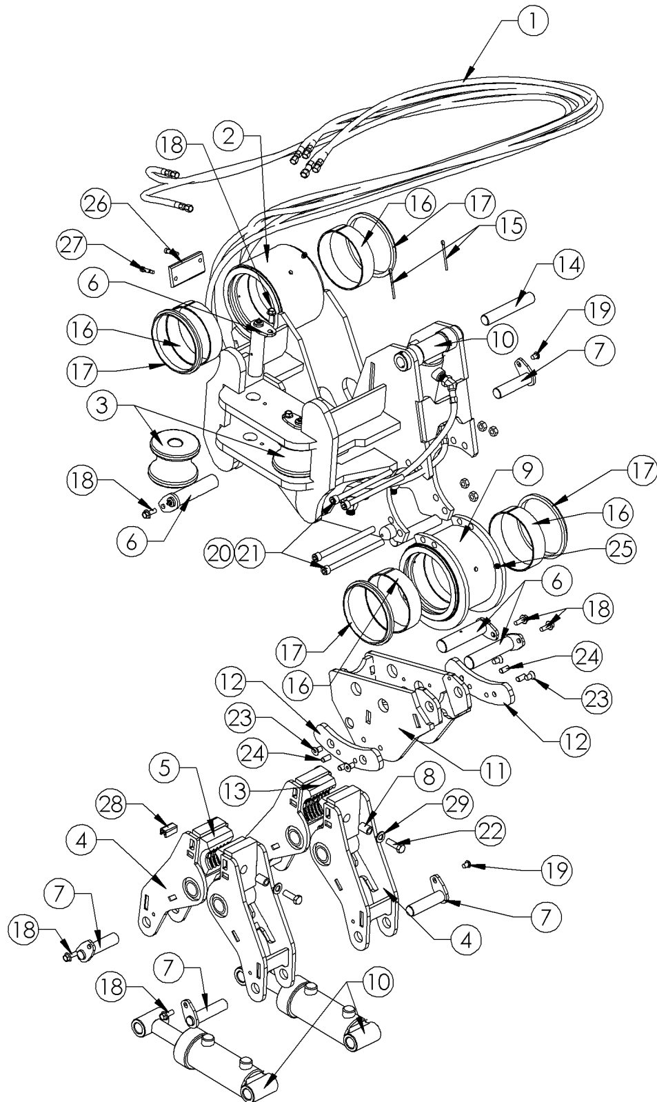
WISE ASSEMBLY FIGURE 40-9
