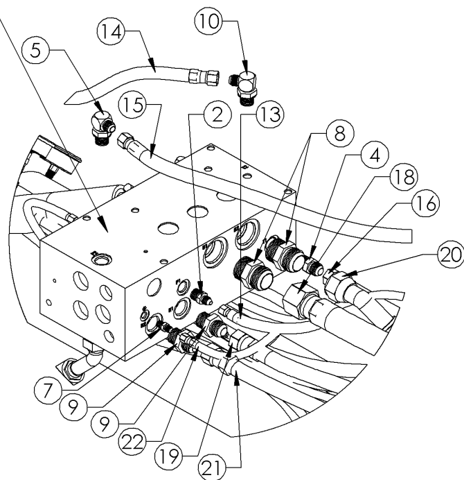
MANIFOLD VALVE TOP VIEW
