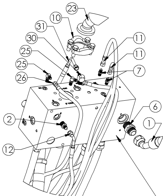
MANIFOLD VALVE BOTTOM VIEW
