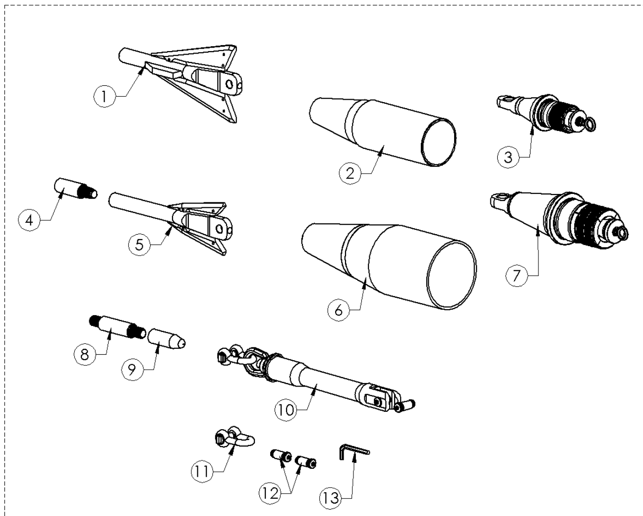
ACCESSORY KIT - INT HB3038 & HB5058
