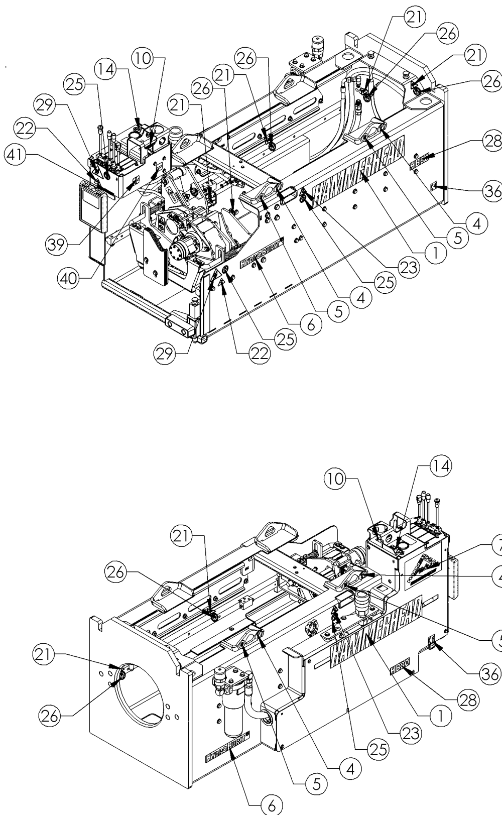
DECAL LOCATIONS - HB80 (INTERNATIONAL) FIGURE 10-5
