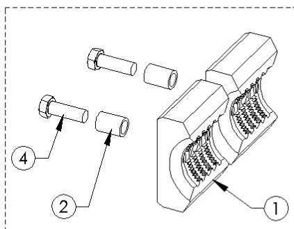
296278-477 FOR HB125, FRONT
