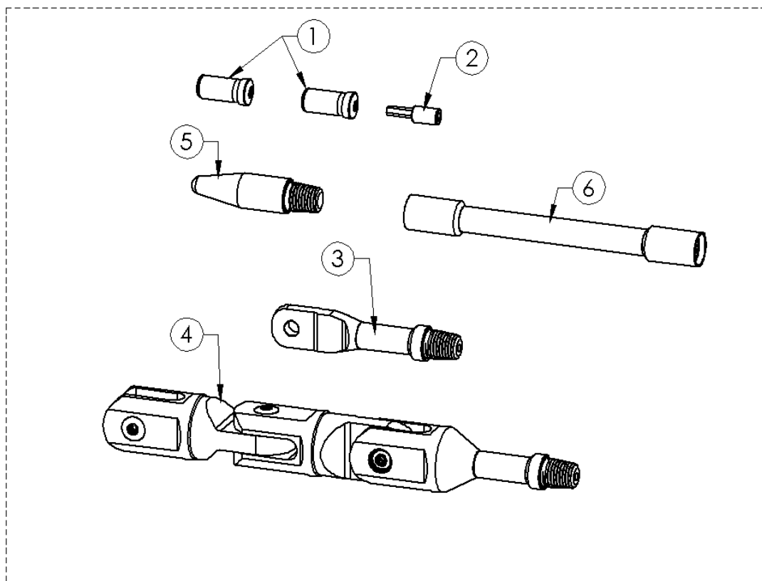
ACCESSORY KIT - HB80
