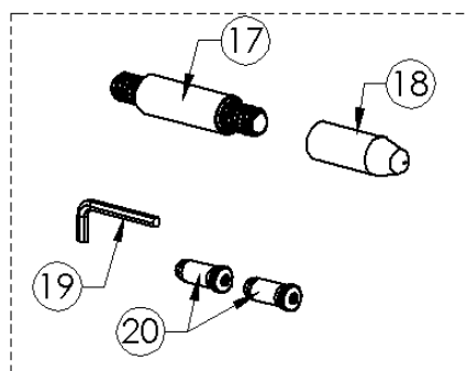
ACCESSORY KIT - DOM HB3038 & HB5058
