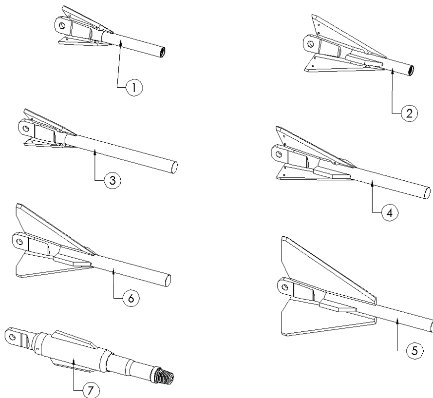
STARTER RODS - BLADED
