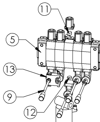
CONTROL VALVE SPACER PLACEMENT
