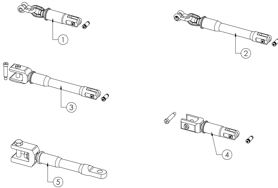
SWIVEL ASSEMBLIES
